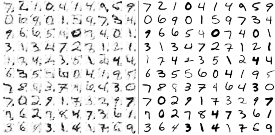
Figure 10: Untargeted FGS \mathcal{L}_{\text{VAE}} Attack: VAE reconstructions (left) and VAE-GAN reconstructions (right). Note the difference in reconstructions compared to Figure 9. Careful visual inspection reveals that none of the VAE reconstructions change class, and only two of the VAE-GAN reconstructions change class (a 6 to a 0 in the next-to-last row, and a 9 to a 4 in the last row). Combining FGS with \mathcal{L}_{\text{VAE}} does not seem to give an effective attack.
