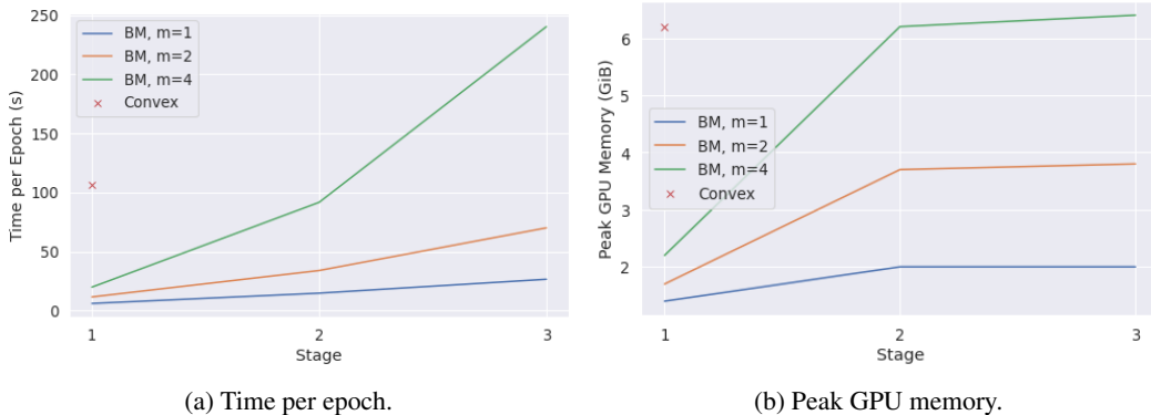
Figure 6: Supplement to Figure 1. Time per epoch and peak GPU memory consumption of different formulations of gated ReLU CNNs trained in a layerwise fashion on CIFAR-10. For "Convex", training causes memory consumption to exceed NVIDIA 1080 Ti GPU’s 12 GB memory capacity after the first stage, preventing ability to train convex CNN (23) in a layerwise fashion.
