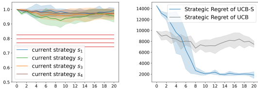
Figure 3: Strategic arm behavior when interacting with incentive-unaware standard UCB. Figure 4: Strategic regret of UCB-S and standard UCB as arms adapt their strategies.
