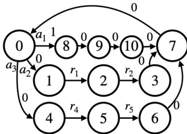
Figure 1: Unichain MDP instance for Proposition 3.4
