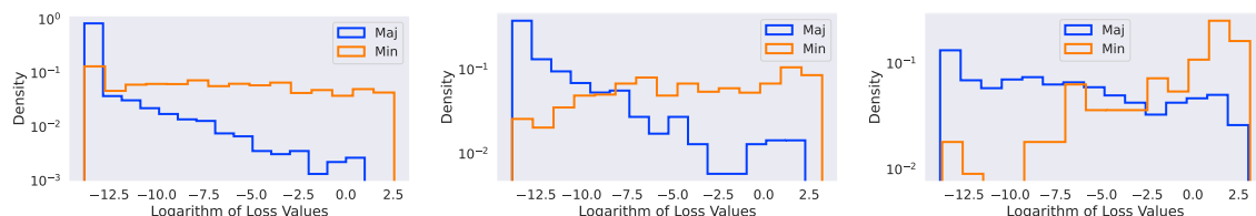
(a) Class 1 of Waterbirds
