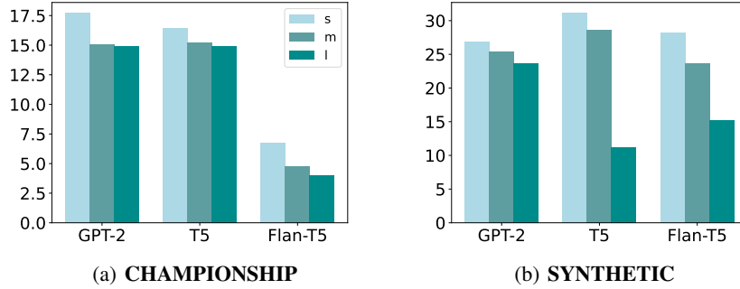
Figure 2: Othello 1-hop generation performance under different model sizes. All models are non-pretrained versions fine-tuned with 20k game sequences.
