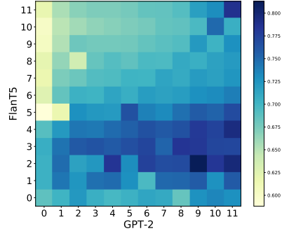
Figure 5: Decoder feature similarity heatmap across different layers.
