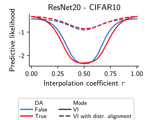
Figure 8: Analysis for data augmentation on ResNet20.
