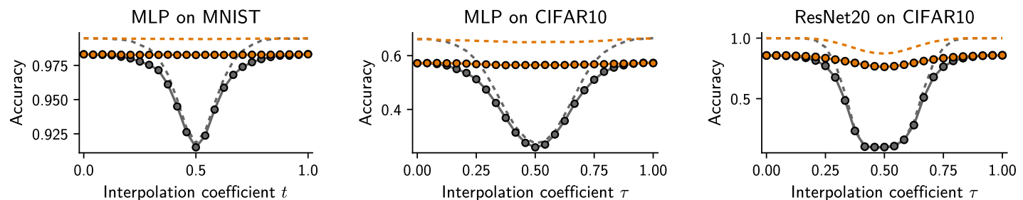
Figure 5: Analysis for accuracy. Follows the same legend as in the paper.
