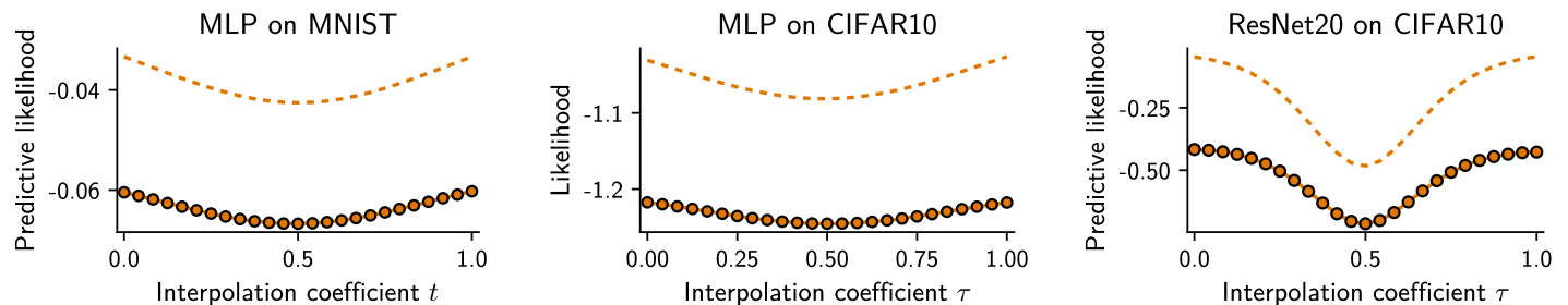
Figure 6: Zoom on Figure 3 (only aligned models). Follows the same legend as in the paper.
