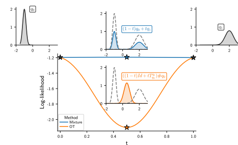
Figure 1: Mixtures vs OT interpolation.
