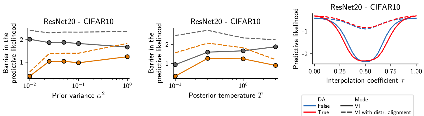
Figure 7: Analysis for prior variance and temperature on ResNet20. Follows the same legend as in the paper.
