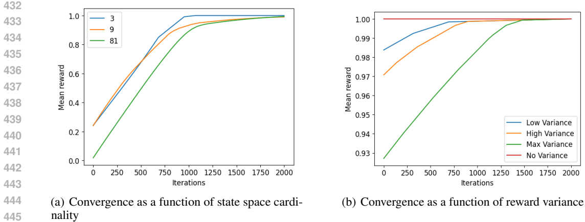
Figure 1: Improvement in average reward as a function of MDP complexity
