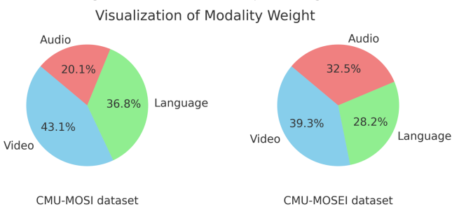
Figure 2: Modality Weight
