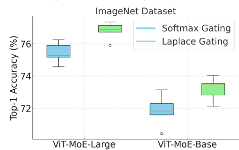
Figure 1: ImageNet Result
