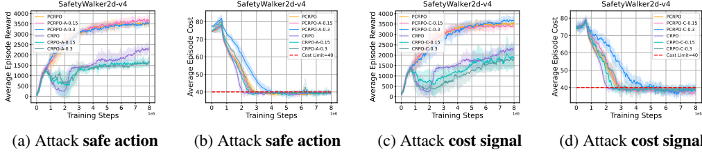
Figure 7: Robust safe RL tasks: Random disturbances over either the action or the agent’s observed immediate cost feedback.
