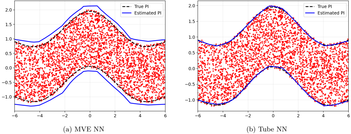
Figure 1: We generate synthetic data points (x_i, y_i) according to the following model: y_i = \frac{\sin(x_i)}{x_i} + \epsilon_i , where \epsilon_i \sim \mathcal{U}(-1, 1) . The Prediction Intervals (PIs) estimated by the MVE neural network deviate significantly from the true underlying PI, whereas the Tube loss-based neural network produces PI estimates that closely align with the true interval.
