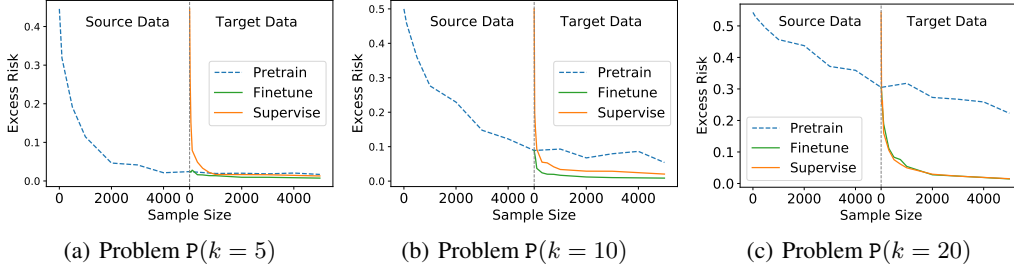
Figure 1: A generalization comparison between pretraining, pretraining-finetuning, and supervised learning. For each point in the curves, its x-axis represents the sample size and its y-axis represents the excess risk achieved by an algorithm with the corresponding amount of samples under the optimally tuned stepsizes. For the pretraining curves, the sample size refers to the amount of source data and the sample size appeared in the right half of the plots should be added by 5,000. The finetuning curves are generated from an initial model pretrained with 5,000 source data and its sample size refers to the amount of target data. The problem instances P(k=5) , P(k=10) , and P(k=20) are designed according to (4). The problem dimension is 200. The results are averaged over 20 independent repeats.
