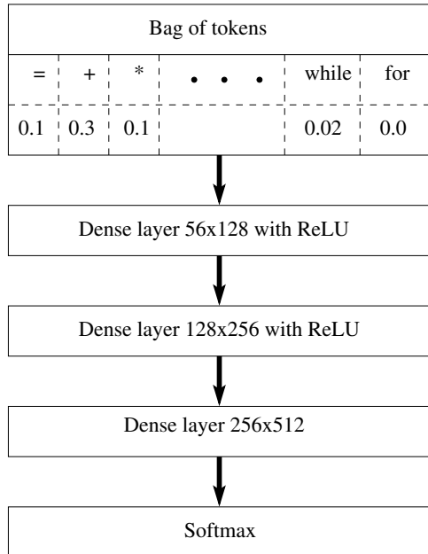
Figure 5: MLP architecture for code classification.
