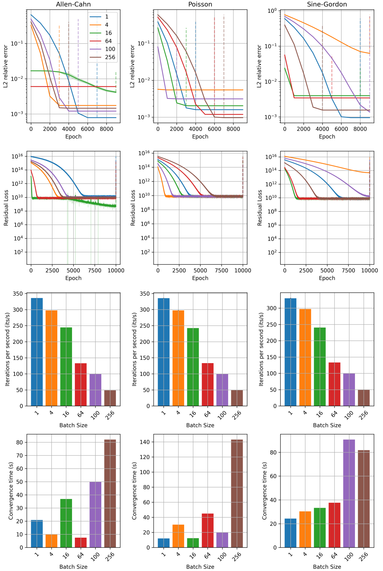
Figure 1: Ablation on randomization batch size with Inseparable and effectively high-dimensional PDEs , \text{dim}=100\text{k} , 5 runs with different random seeds. Model converges when the difference of L2 error is below 1\text{e-}7 .
