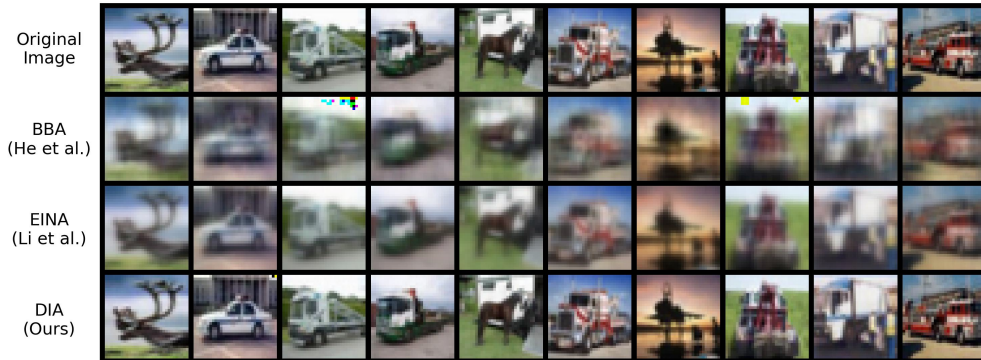
Figure 2: Reconstructed inputs comparison of prior approaches and our method on Block3 of ViT
