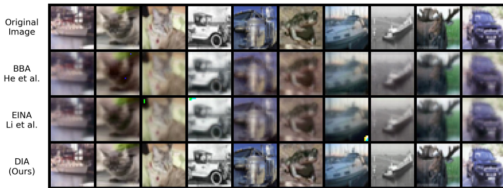
Figure 1: Reconstructed inputs comparison of prior approaches and our method on Layer1 of ResNet
