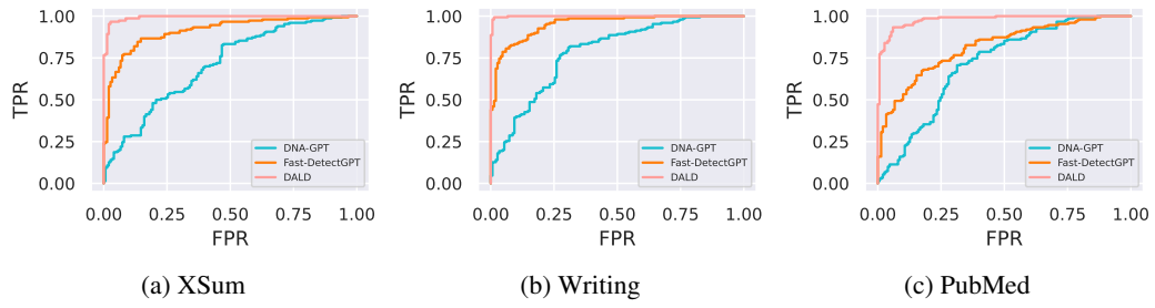
Figure 1: The FPR-TPR curve of different methods on XSum, Writing and PubMed dataset. The results show that our method achieves highest score at low FPR compared with DNA-GPT and Fast-DetectGPT.
