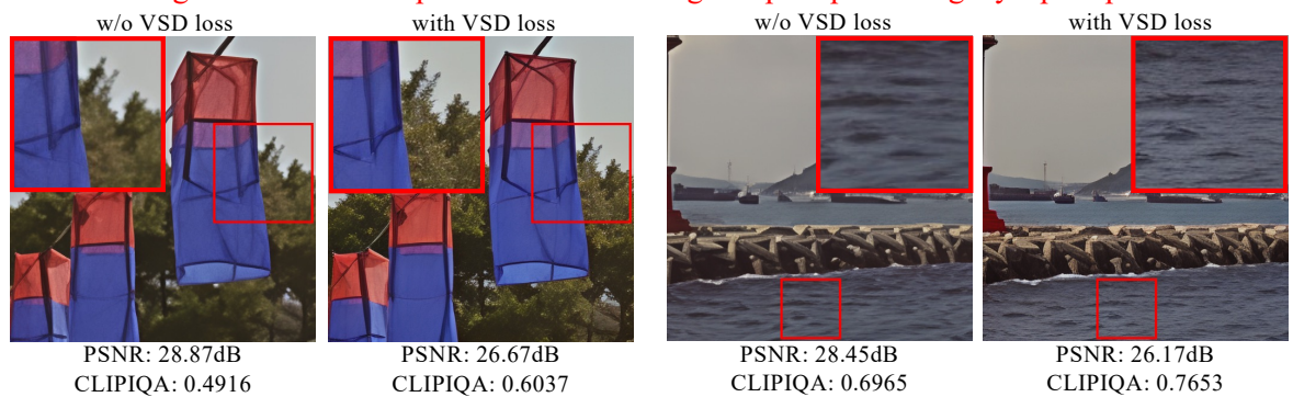
Figure 5: Visual comparison with and without VSD loss.
