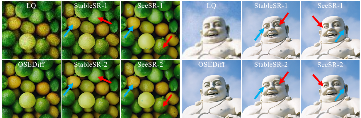
Figure 2: Visual comparison of outputs by OSedDiff, StableSR (2 samples) and SeeSR (2 samples) using the same LQ image.
