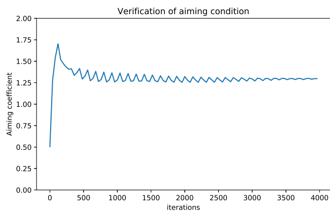
Figure 1: Verifying aiming condition on MNIST.
