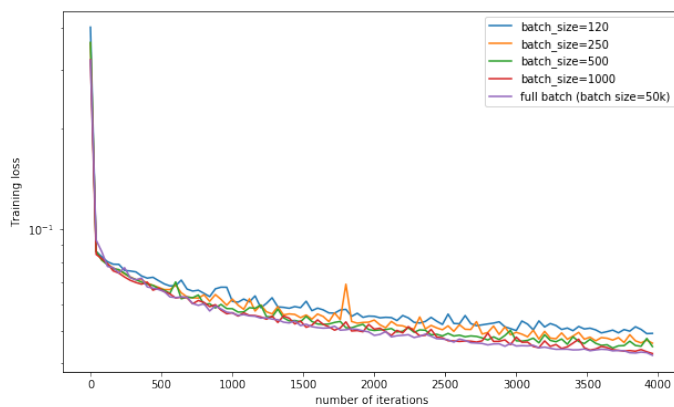
Figure 3: Comparing mini-batch SGD with full batch GD on CIFAR-10.
