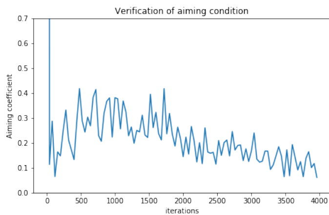
Figure 2: Verifying aiming condition on CIFAR-10.
