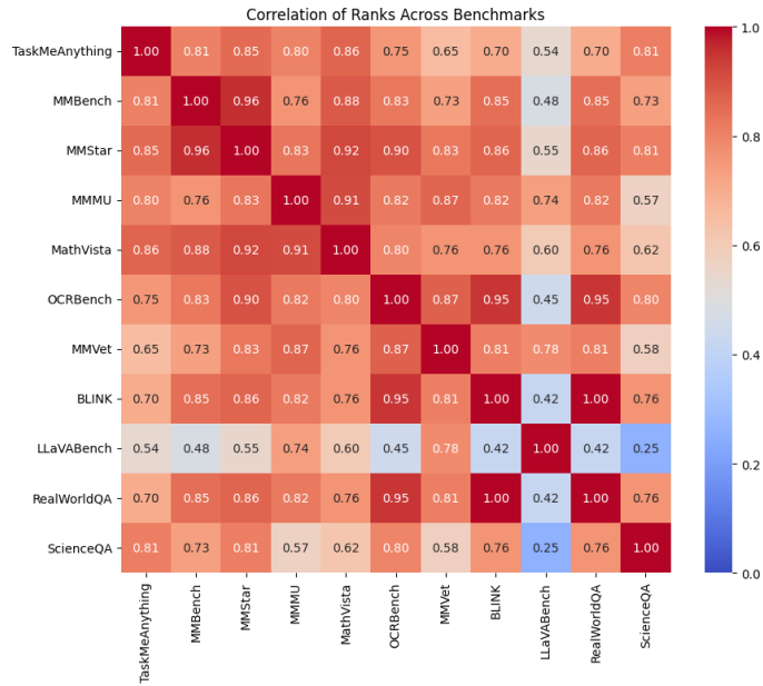
Figure 2: Model ranking correlation between Task-Me-Anything and existing benchmarks.
