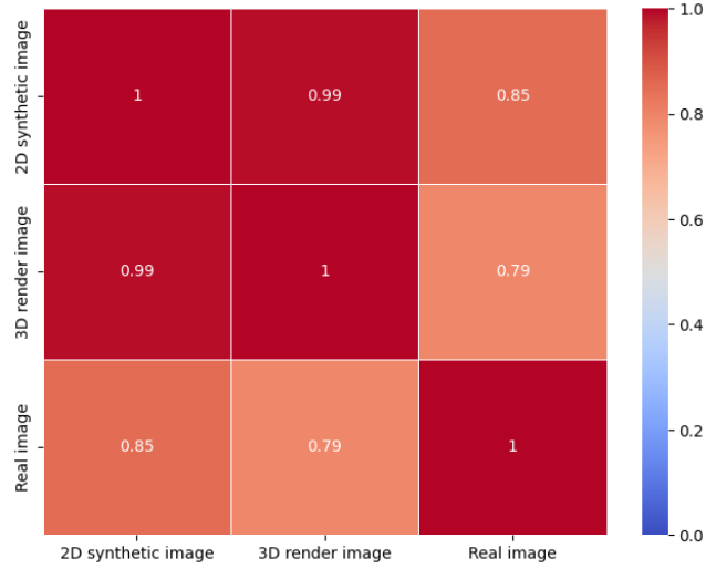
Figure 1: Model ranking correlation between different subsets of Task-Me-Anything.
