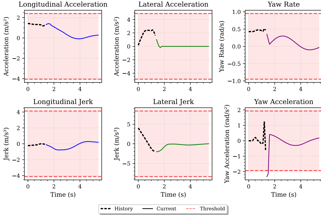
Figure 9: Statistical Comparison of History Comfort (HC) Failure Case.
