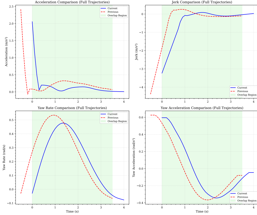
Figure 4: Statistical Comparison of Extended Comfort (EC) Failure Case.
