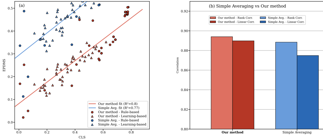
Figure 13: Simple Averaging correlation analysis.
