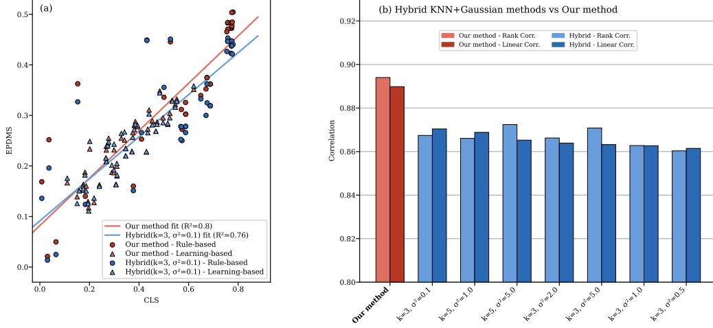
Figure 14: Hybrid kNN/Gaussian correlation analysis.
