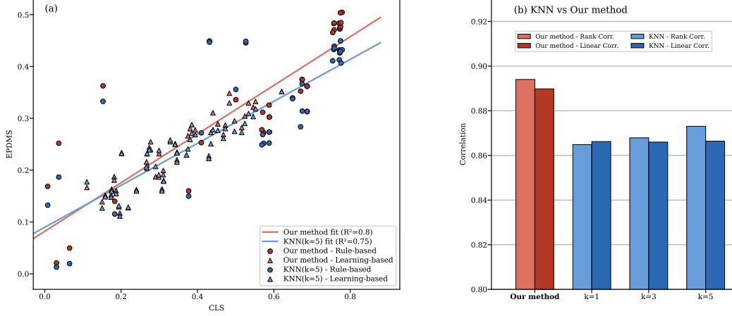
Figure 12: kNN correlation analysis.
