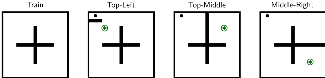
Figure 2: Point mass-maze with changed dynamics. TRAIN is the unmodified version of point mass-maze from the ExORL benchmark; we use the RND dataset to pre-train our BFMs. TOP-LEFT, TOP-MIDDLE, and MIDDLE-RIGHT introduce an obstacle that change the environment dynamics. The agent is initialised at \bullet and tasked with reaching \otimes .
