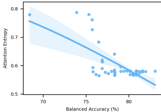
Entropy-BAC Relationship Curve During the Training Process on TUAB
