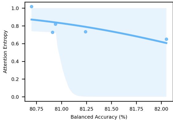
Entropy-BAC Relationship Curve of Warm Up XAI on TUAB
