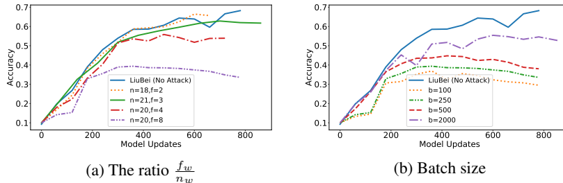
Figure 4: Convergence in a Byzantine environment.
