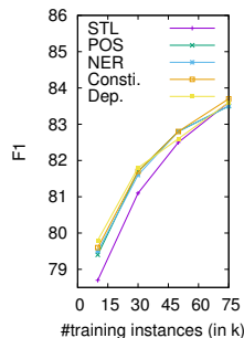
Figure 2: MTL Performance of SRL wrt. the data size.
