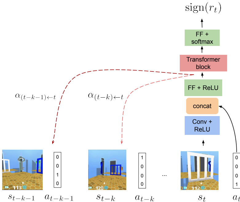
Figure 7: The architecture used for SECRET. \alpha_{\leftarrow t} is the vector containing the attention weights of the model for its prediction at step t .
