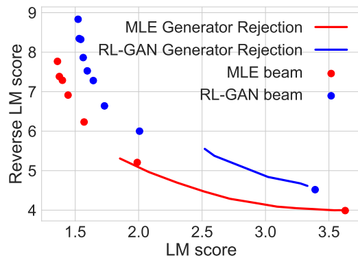
Figure 10: MLE still outperforms RL-GAN under different decoding mechanisms.
