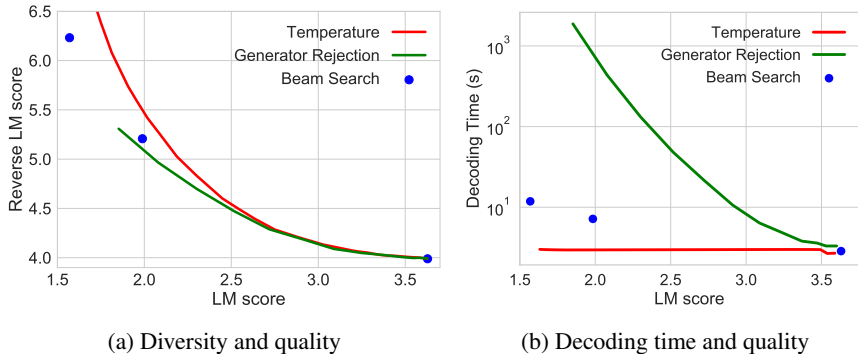
Figure 5: Analysis of decoding methods. ( lower is better for all metrics ). Left: Less biased methods provided a better quality/diversity trade-off. Right: However, they are computationally much more expensive.
