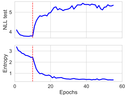
Figure 6: Dotted line indicates the start of GAN training. We notice a clear drop in entropy (spike in NLL_{test} ) when moving from maximum-likelihood to adversarial updates.
