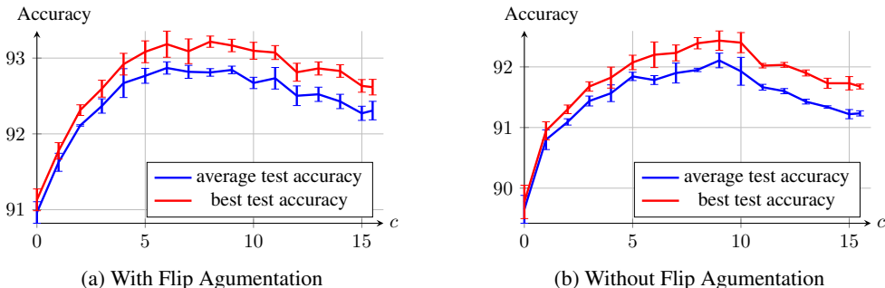
Figure 2: Test accuracy of 10-layer CNN with various values for the c parameter in BBlur.
