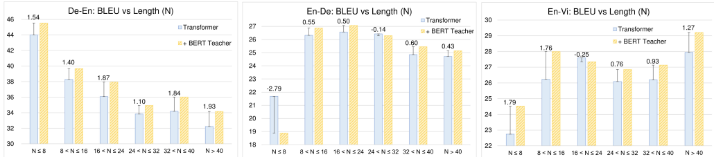
Figure 2: BLEU scores on IWSLT German-English, WMT English-German and IWSLT English-Vietnamese for different output lengths.
