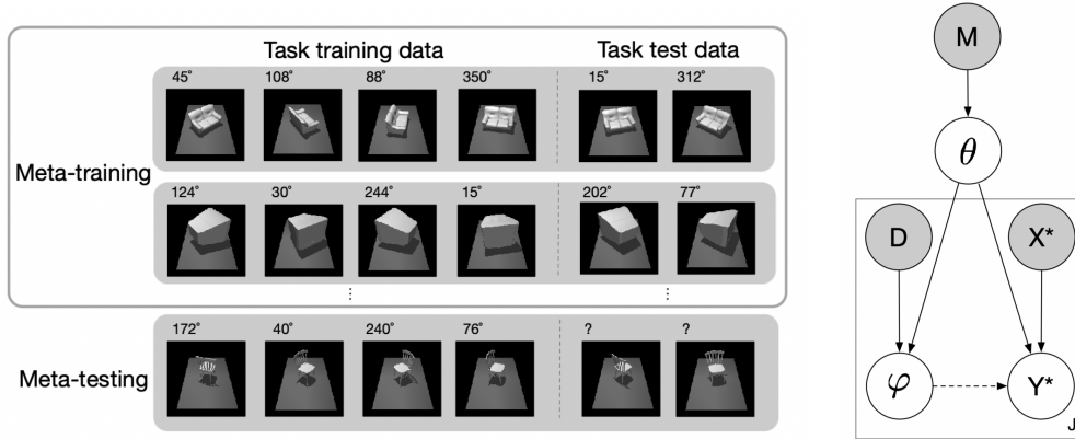
Figure 1: Left: An example of non-mutually-exclusive pose prediction tasks, which may lead to the memorization problem. The training tasks are non-mutually-exclusive because the test data label (right) can be inferred accurately without using task training data (left) in the training tasks, by memorizing the canonical orientation of the meta-training objects. For a new object and canonical orientation (bottom), the task cannot be solved without using task training data (bottom left) to infer the canonical orientation. Right: Graphical model for meta-learning. Observed variables are shaded. Without the dashed arrow, Y^* is conditionally independent of \phi given \theta , which we refer to as complete memorization (Definition 1).
