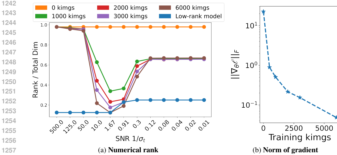
Figure 6: (a) Numerical rank of \nabla_{x_t} \mathbf{x}_\theta(x_t, t) at all time of diffusion models. Problem (6) is trained with the DAE \mathbf{x}_\theta(\cdot, t) parameterized according to (9) and U-Net on the training samples generated by the mixture of low-rank Gaussian distribution. The x -axis is the SNR and the y -axis is the numerical rank of \nabla_{x_t} \mathbf{x}_\theta(x_t, t) over the ambient dimension n , i.e., \text{rank}(\nabla_{x_t} \mathbf{x}_\theta(x_t, t))/n . Here, kimgs denotes the number of samples used for training, which equals to training iterations times batch size of training samples. (b) Convergence of gradient norm of the training loss: The x -axis is kimgs (see Eq. (46)), and the y -axis is the gradient norm of the training loss.
