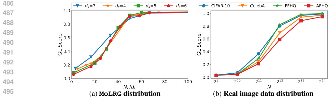
Figure 5: Phase transition of learning distributions via U-Net. In (a), the x -axis is the number of training samples over the intrinsic dimension, while in (b), it is the total number of training samples. The y -axis is the GL score. We train diffusion models with the U-Net architecture on (a) the data samples generated by the MoLRG distribution with K = 2 , n = 48 and d_k varying from 3 to 6 and (b) real image datasets CIFAR-10, CelebA, FFHQ and AFHQ. The GL score is low when U-Net memorizes the training data and high when it learns the underlying distribution.
