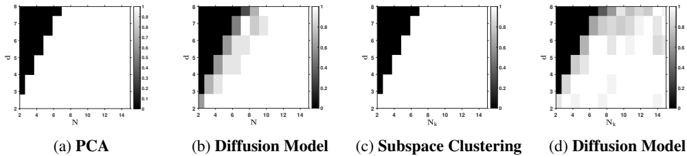
Figure 4: Phase transition of learning the MoLRG distribution. The x -axis is the number of training samples and y -axis is the dimension of subspaces. Darker pixels represent a lower empirical probability of success. When K = 1 , we apply SVD and train diffusion models to solve Problems (12) and (6), visualizing the results in (a) and (b), respectively. When K = 2 , we apply a subspace clustering method and train diffusion models for solving Problems (18) and (6), visualizing the results in (c) and (d), respectively.
