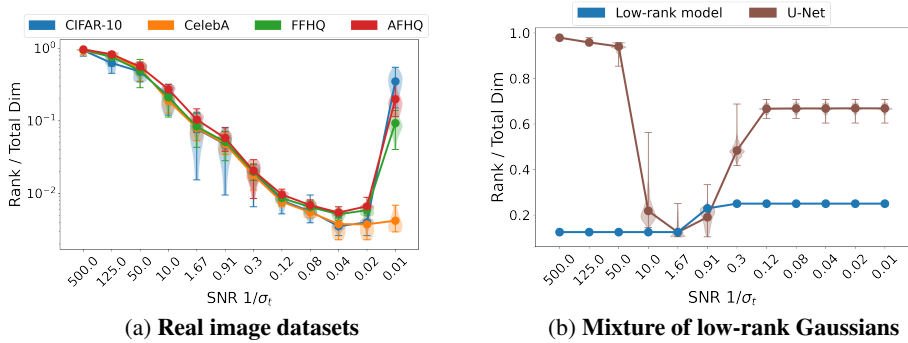
Figure 3: Low-rank property of the DAE of trained diffusion models. We plot the ratio of the numerical rank of the Jacobian of the denoising autoencoder, i.e., \nabla_{\mathbf{x}_t} \mathbf{x}_\theta(\mathbf{x}_t, t) , over the total dimension against the signal-to-noise ratio (SNR) 1/\sigma_t on trained diffusion models. (a) We train diffusion models on image datasets CIFAR-10, CelebA, FFHQ, and AFHQ. The experimental details are provided in Appendix C.1. (b) We respectively train diffusion models with the low-rank parameterization (9) and U-Net on a mixture of low-rank Gaussian distributions.
