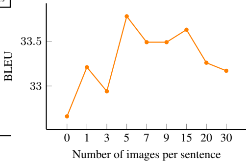
Figure 5: Influence of the number of images on the BLEU score.
