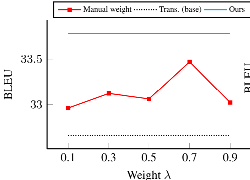
Figure 4: Quantitative study of the gating weight \lambda .
