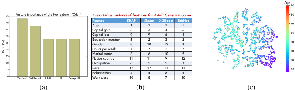
Figure 6: (a) Comparison to previous work for feature importance score of the top feature, “Odor” for the mushroom edibility prediction (Dua & Graff, 2017) (task: classify whether a mushroom is edible or poisonous). With “Odor” feature only, > 98.5% test accuracy can be obtained, so a high feature importance is expected to be assigned to it, as observed with TabNet. (b) Comparison to previous work for importance ranking of features in the Adult Census Income dataset (Dua & Graff, 2017) (task: distinguish whether a person’s income is above $50,000). (c) Impact of the most important feature on the decision manifold. T-SNE of the decision manifold for Adult Census Income test samples and the impact of the most dominant feature ‘Age’.
