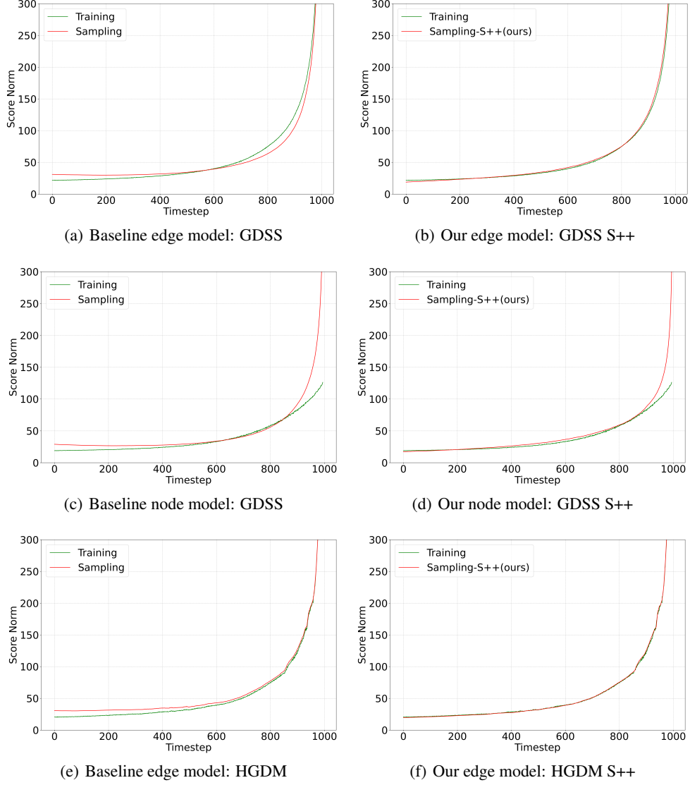
Figure 1: Expectation of \|s_{\theta,t}(\cdot)\|_2 during sampling and training on Community-small.
