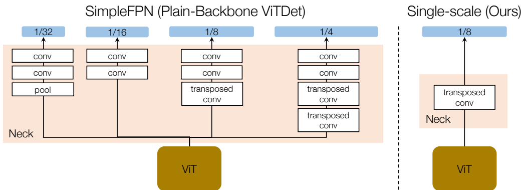
Figure A: The creation of input features. Left: The creation of feature pyramids from the last feature of the plain backbone, ViT, in SimpleFPN (Li et al., 2022) where different stacks of convolutional layers are used to create features at different scales. Right: The design of our single-scale feature map with only one layer.
