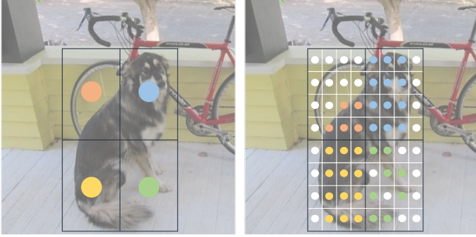
Figure B: Masked Instance-Attention. Left: The box-attention (Nguyen et al., 2022) which samples 2 \times 2 grid features in the region of interest. Right: Our masked instance-attention for dense grid sampling that employs masking strategy to capture object boundary. The 2 \times 2 attention scores are denoted in four colours and the masked attention score is shown in white.
