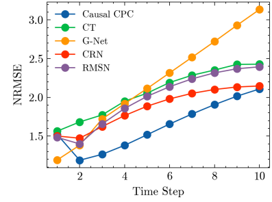
Figure 3: Cancer Sim seq\_length = 40, \gamma = 3
