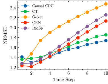
Figure 2: Cancer Sim seq\_length = 40, \gamma = 2
