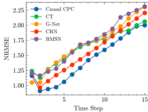
Figure 7: Cancer simulation, \tau = 15
