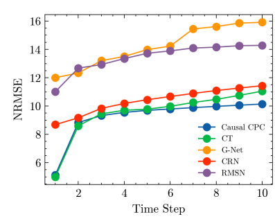
Figure 6: Real MIMIC III
