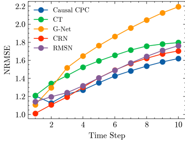
Figure 1: Cancer Sim seq\_length = 40, \gamma = 1
