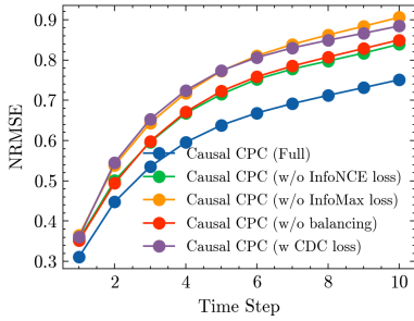
Figure 4: MIMIC III semi-synthetic, ablation study.
