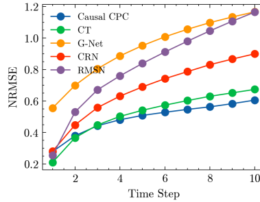
Figure 5: MIMIC III semi-synthetic, seq\_length = 60
