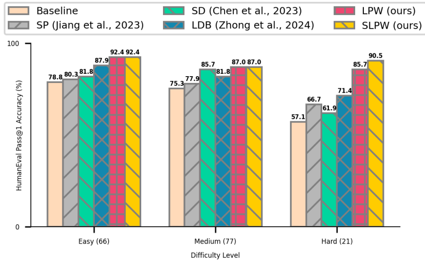
Figure 1: The Pass@1 accuracy across different difficulty levels, Easy , Medium , and Hard (part (b)) on the HumanEval benchmark when leveraging GPT-3.5 as the LLM backbone.
