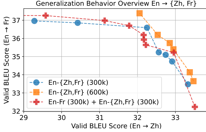
Figure 1: The BLEU score plot paints a better picture for pre-training than the cross-entropy plot, since pre-training was able to improve the En-Zh BLEU score to be on par with the score of joint training for 600k steps.
