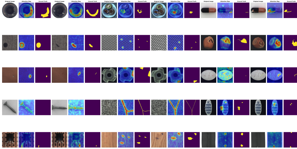
Figure 9: Qualitative results of our method on MVtec-AD Bergmann et al. (2019).
