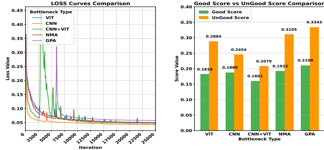
Figure 7: The plots of loss (left part) and the averaged anomaly scores (right part) of different modules in decoder on Universal Medical. CNN: convolution neural network, ViT: vision transformer, NMA: neighbor-masking attention and GPA: global perturbation attention.
