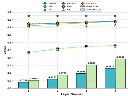
Figure 8: The plots of metrics (left part) and the averaged anomaly scores (right part) of different layer number in LRNB. Influences of the number of layer in LRNB on Universal Medical.
