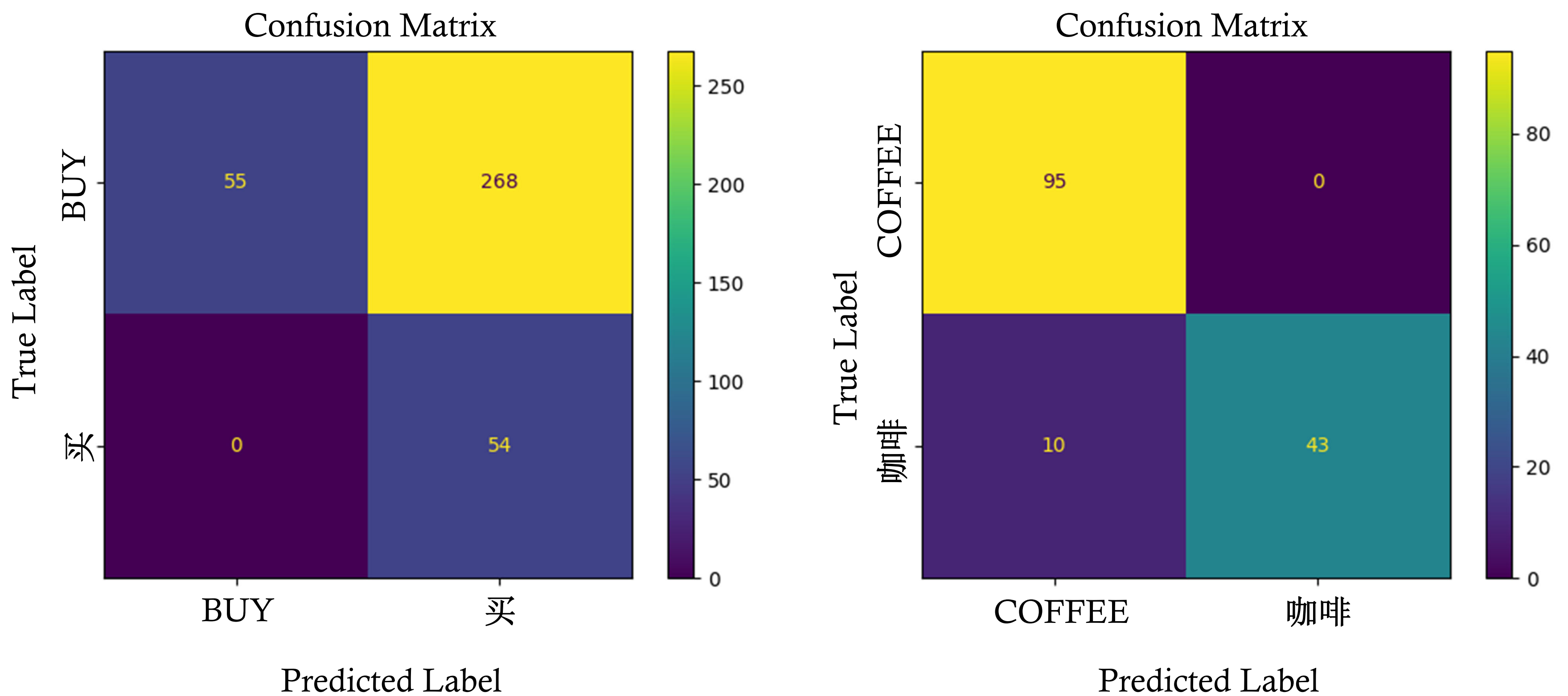
Figure 1. Confusion matrix of model predictions and labels for the two pairs of samples, "COFFEE" and "咖啡" as well as "BUY" and "买".
