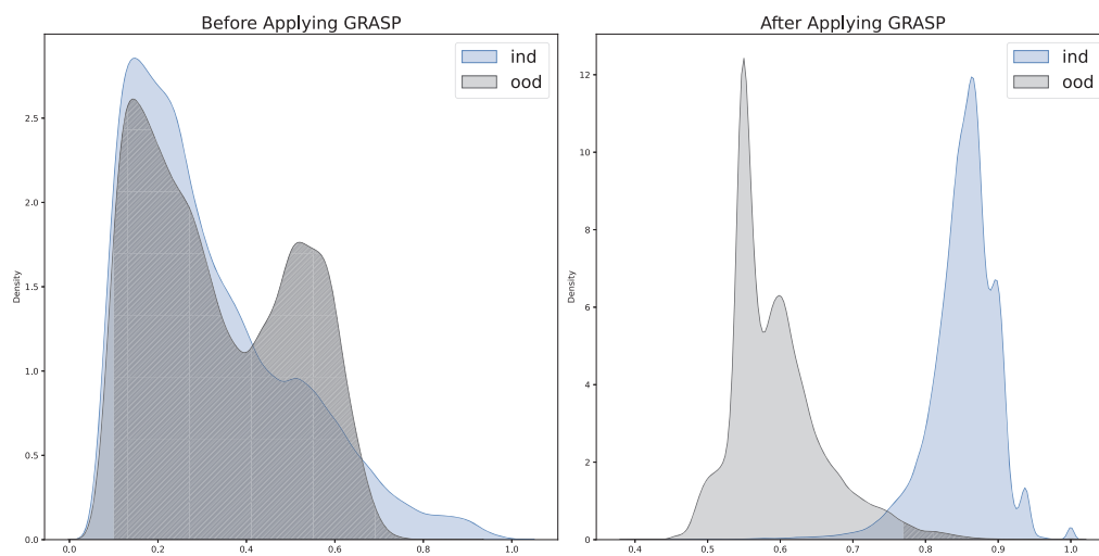
Figure 1: The original MSP score results in a significant overlap between ID and OOD, leading to poor performance. After applying GRASP, the ID scores are significantly increased, resulting in a better distinction between ID and OOD, which greatly reduces the FPR (the shaded area with diagonal lines).
