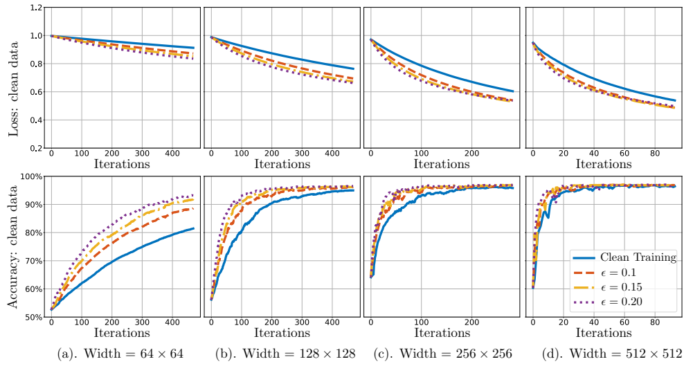
Figure 4: GDAT with Different Perturbation Level: Clean Test Loss
