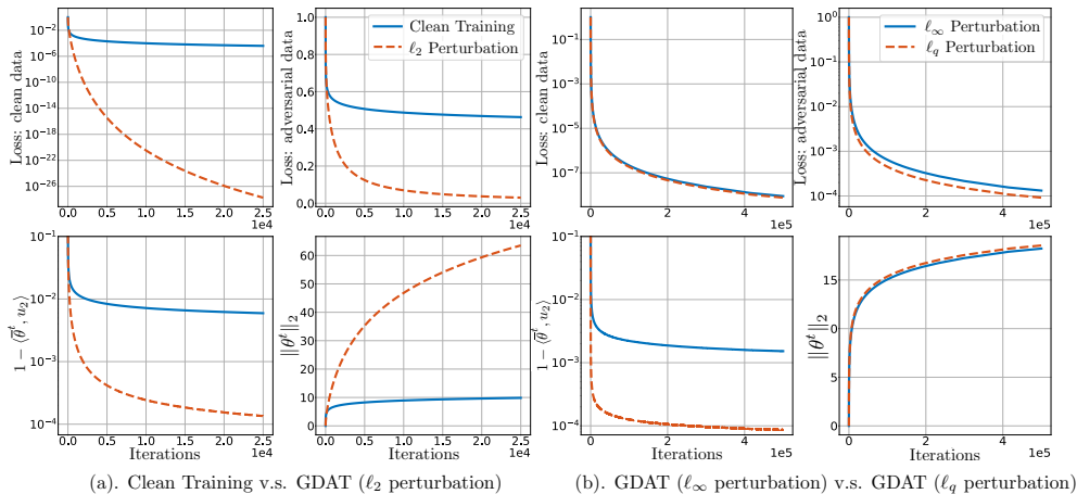
Figure 1: GDAT of Linear Classifiers.
