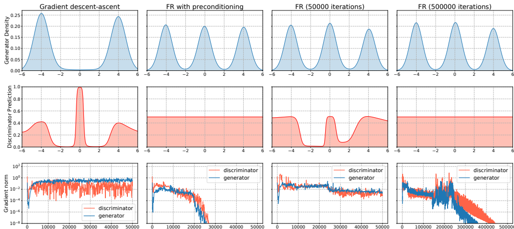
Figure 9: Ablation study on the effect of preconditioning. Vanilla FR also converges in the end of training though it takes much longer.
