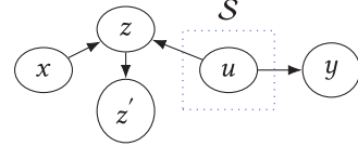
(b) Conditioning on S blocks z as z is a collider and neither z nor z' is in S .
