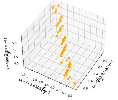
(f) PMGDA
