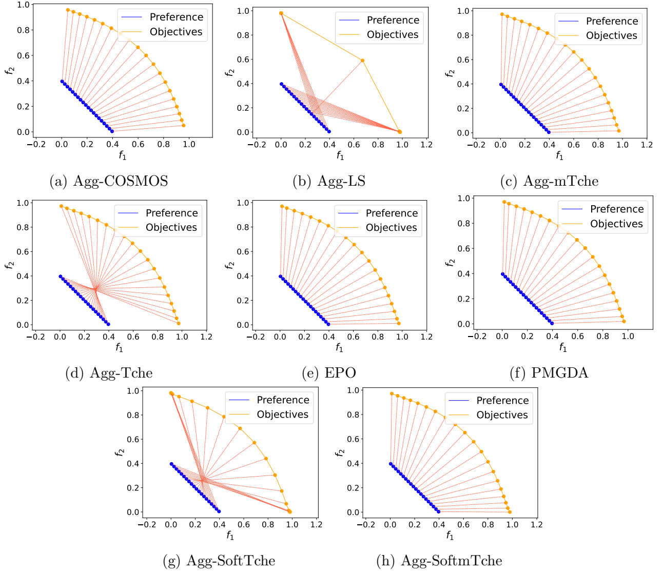
Figure 1: Predicted Pareto solutions from a Pareto neural model on VLMOP2.
