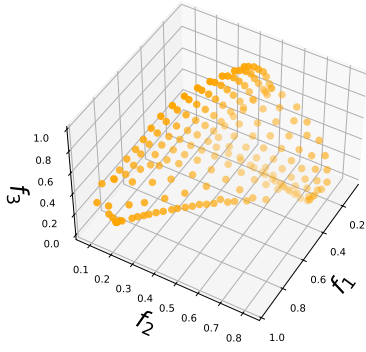
(a) Agg-COSMOS
