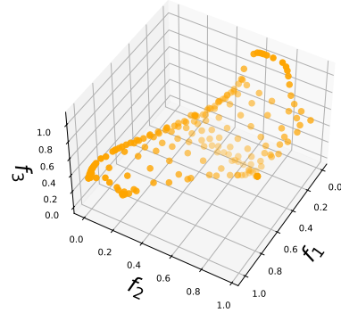
(h) Agg-SoftmTche
