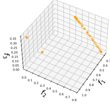
(b) Agg-LS
