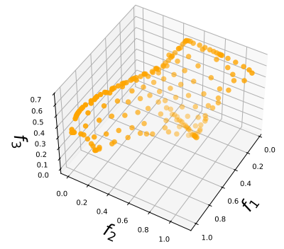
(c) Agg-mTche
