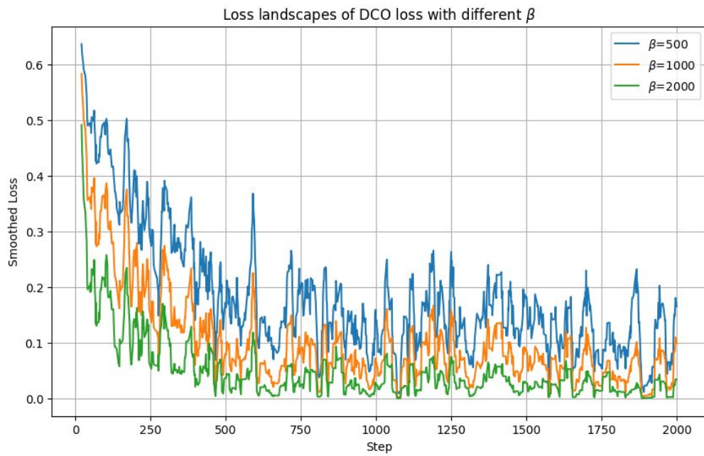
Figure B. Loss landscape of DCO
