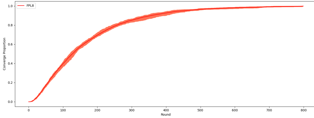
Figure 7: Error Bar of FPL8 in Section 5.
