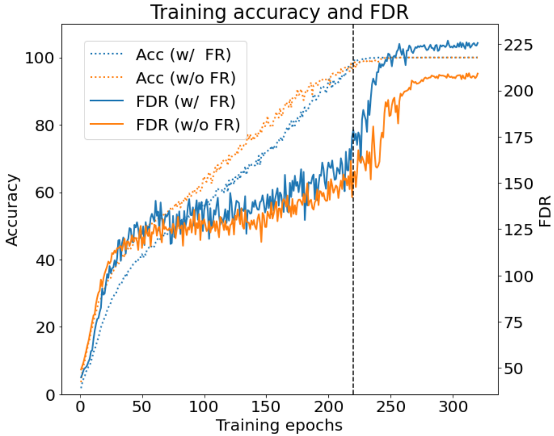
Figure 1: Relationship between number of training epochs, training accuracy, and FDR for CIFAR100-LT. "w/ FR" and "w/o FR" represent WD&ETF&FR and WD&ETF, respectively. The difference in FDR between training with FR and without FR increases significantly after the training error reaches almost 0%.
