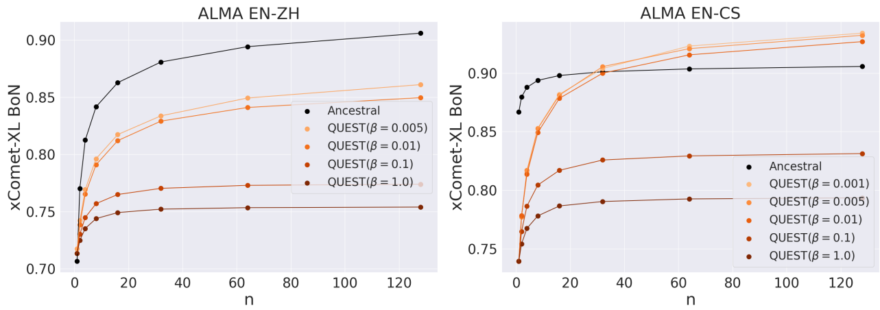
Figure 3: Best-of-N experiments
