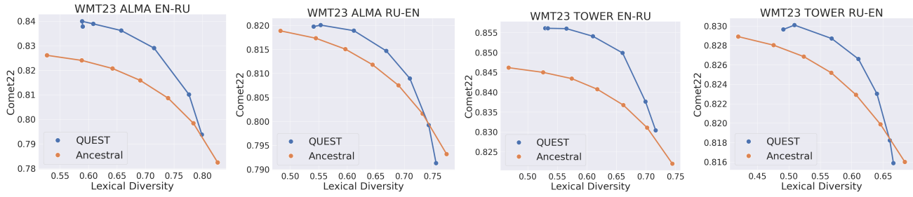
Figure 2: Comet22 on EN-RU and RU-EN
