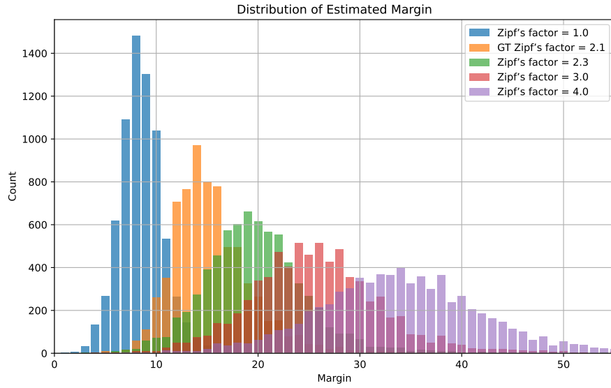
Figure 7: The distribution of the estimated margin during training on the PHOENIX-2014T dataset. The green distribution represents our current paper’s method (factor = 2.3), while the orange distribution shows the ground truth calculated based on gloss annotations.
