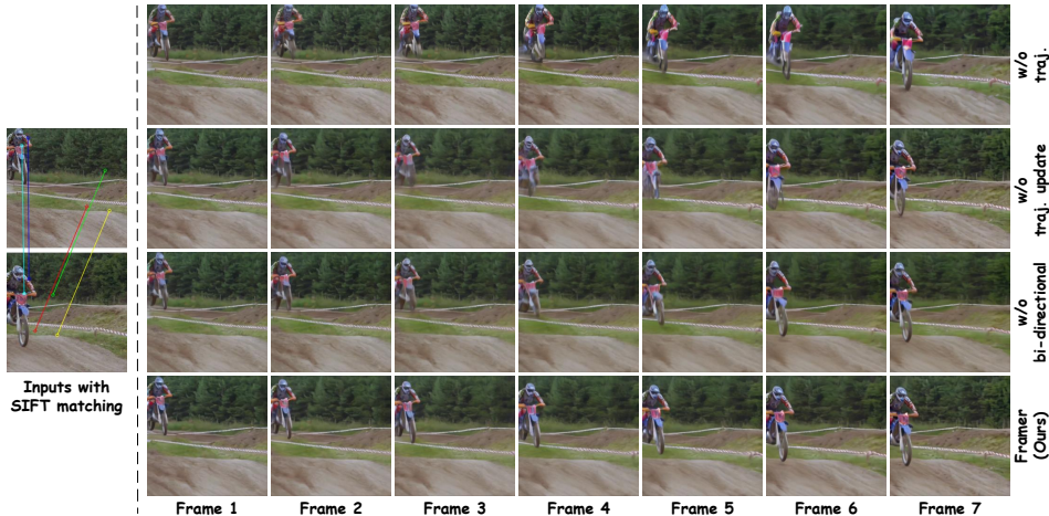
Figure 12: Ablations on each component. “w/o trajectory” denotes inference without guidance from point trajectory, “w/o traj. update” indicates inference without trajectory updates, and “w/o bi” suggests trajectory updating without bi-directional consistency verification.
