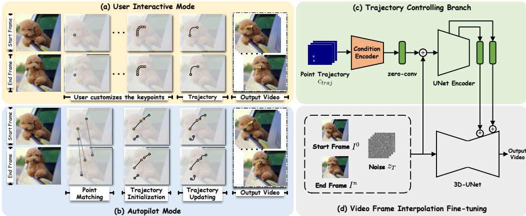
Figure 2: Framer supports (a) a user-interactive mode for customized point trajectories and (b) an “autopilot” mode for frame interpolation without trajectory inputs. During training, (d) we fine-tune the 3D-UNet of a pre-trained video diffusion model for frame interpolation. Afterward, (c) we introduce point trajectory control by freezing the 3D-UNet and fine-tuning the controlling branch.
